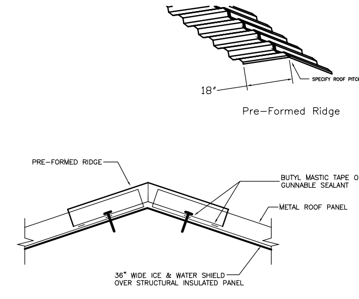
5 TYPICAL RIDGE DETAIL NO SCALE
