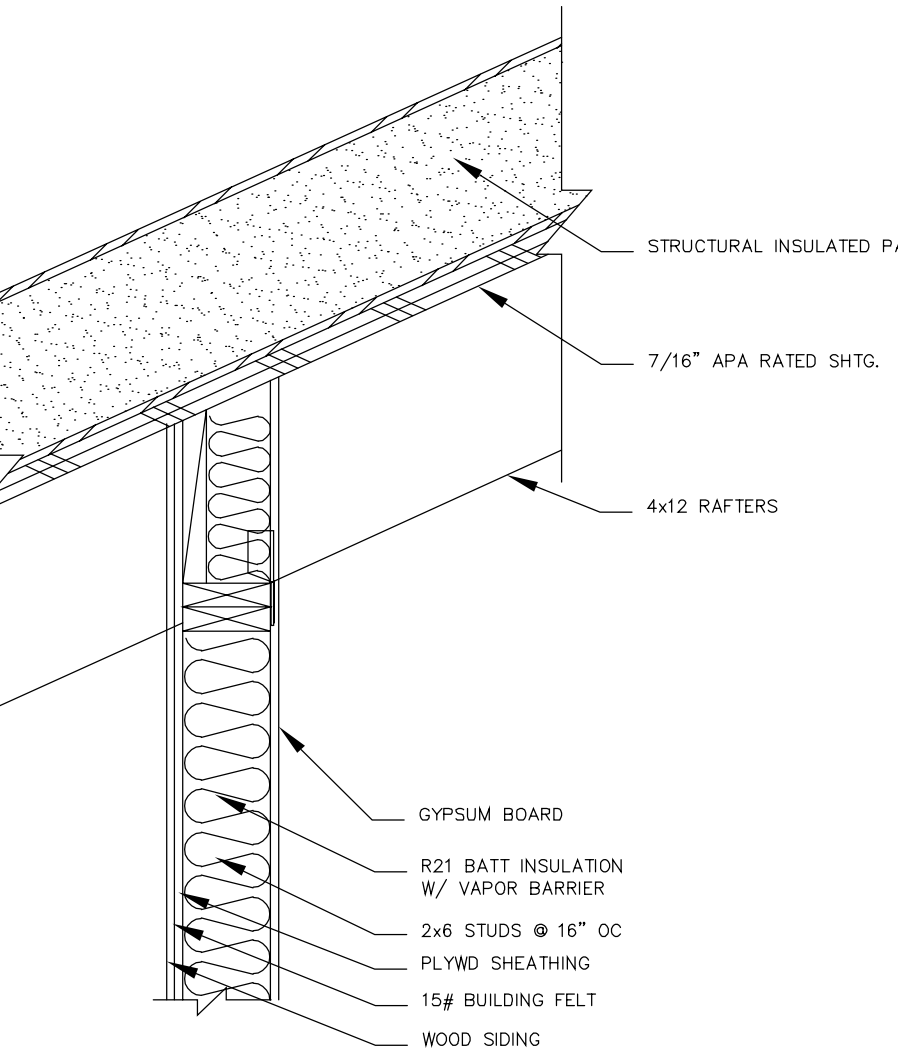
9 ROOF @ EXTERIOR WALL TOP PLATE NO SCALE
