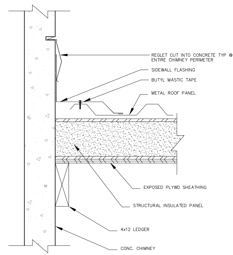
10 ROOF @ CHIMNEY DETAIL NO SCALE
