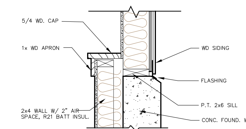
11 FOUNDATION TO STUD WALL DETAIL NO SCALE
