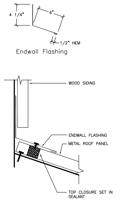
7 TYPICAL ROOF TO END WALL DETAIL NO SCALE
