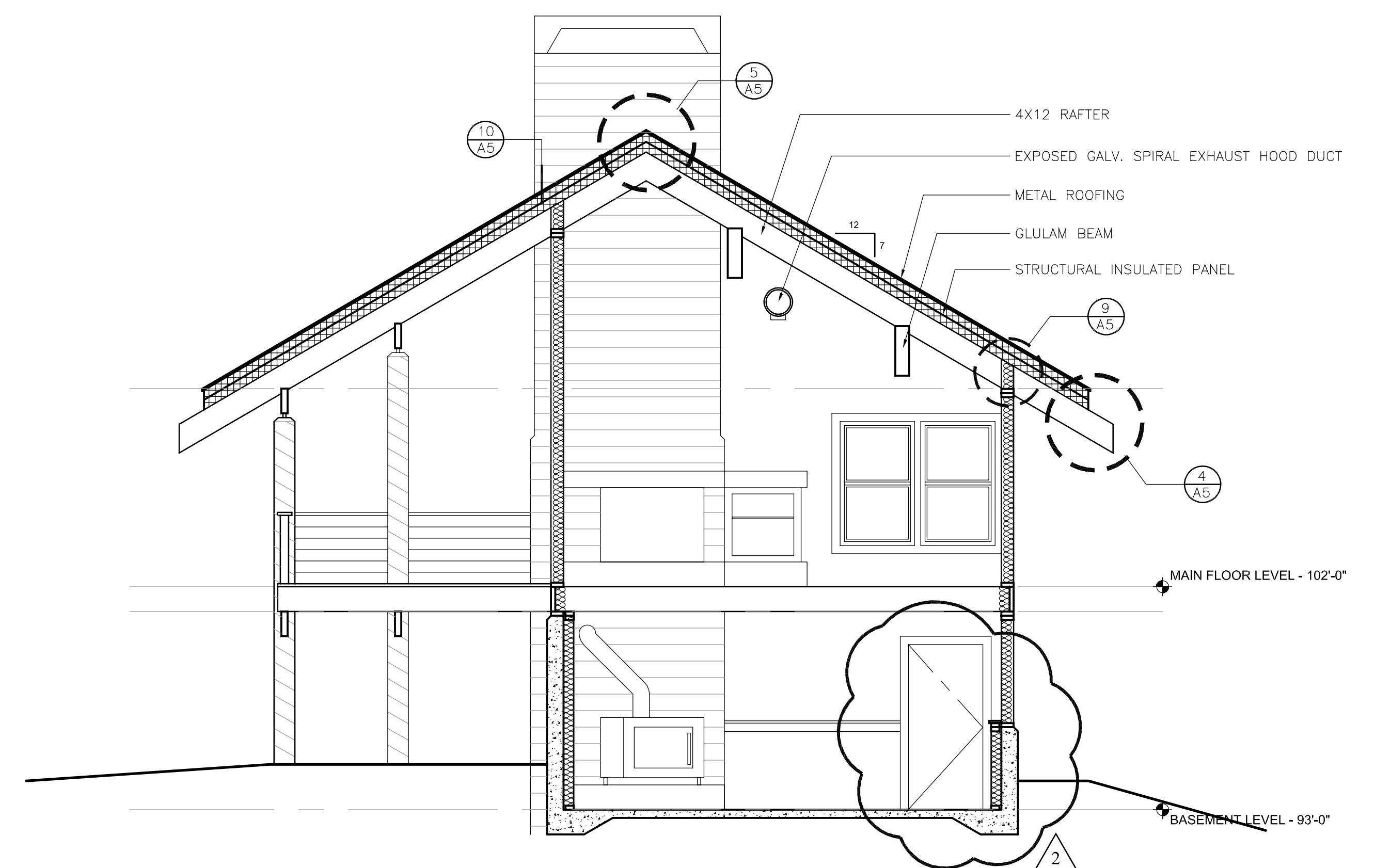
2 CROSS SECTION 1/4" = 1'-0"
