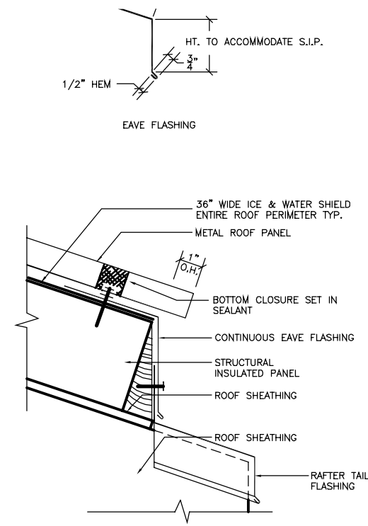
4 TYPICAL EAVE DETAIL NO SCALE
