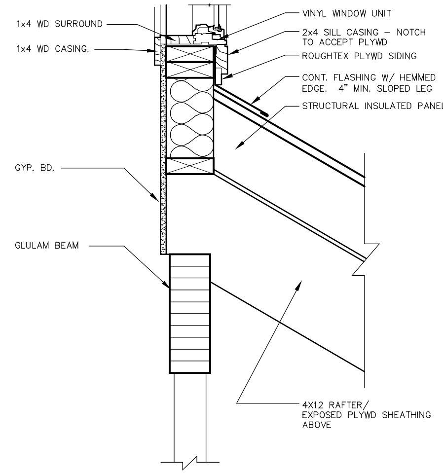
6 ROOF @ CLERESTORY SILL DETAIL NO SCALE
