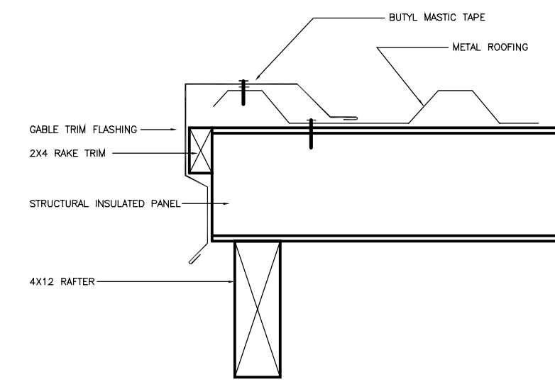
3 TYPICAL GABLE END DETAIL NO SCALE
