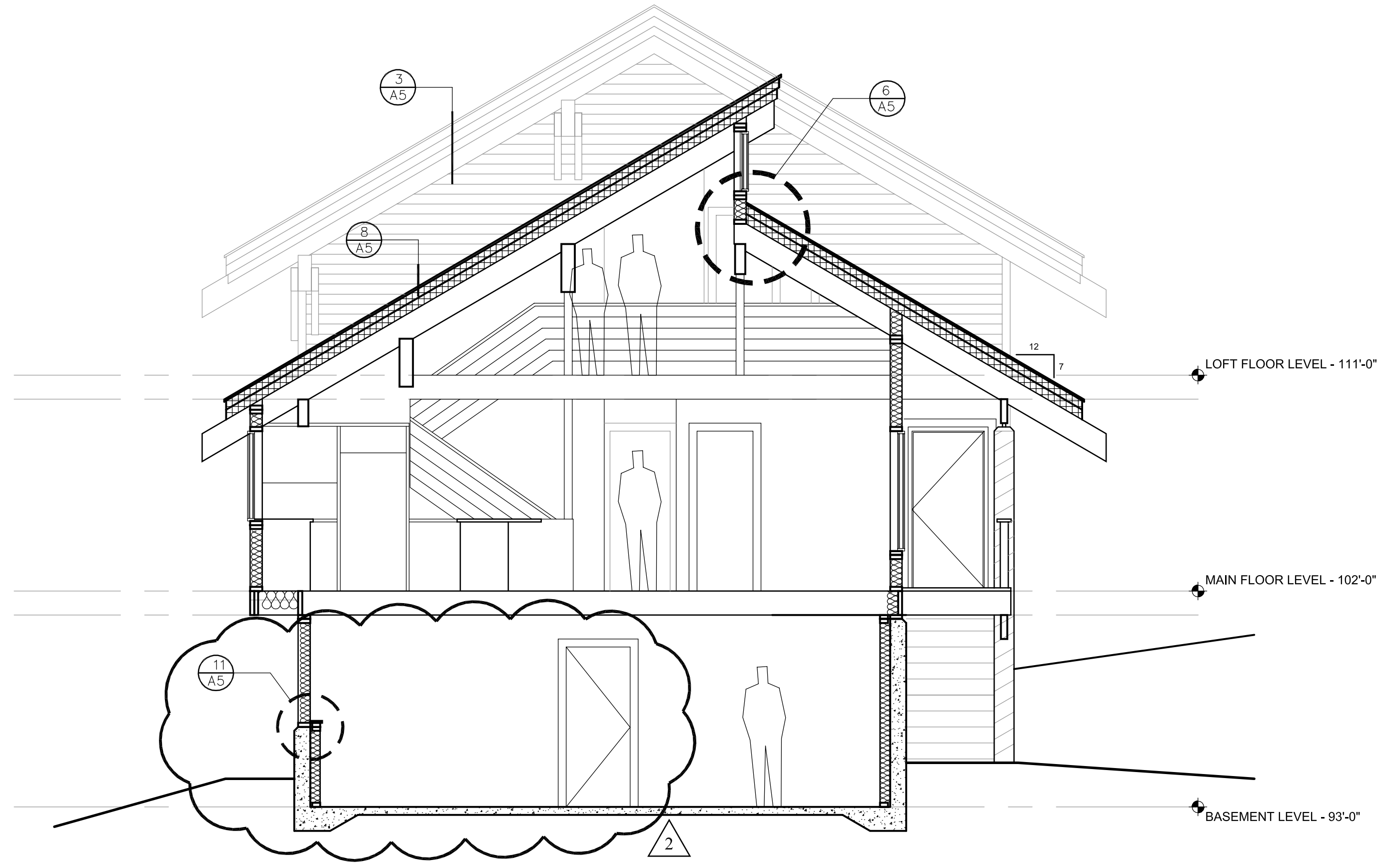
1 CROSS SECTION 1/4" = 1'-0"
